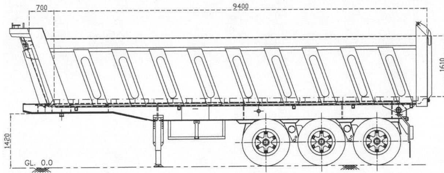
SIDE ELEVATION
